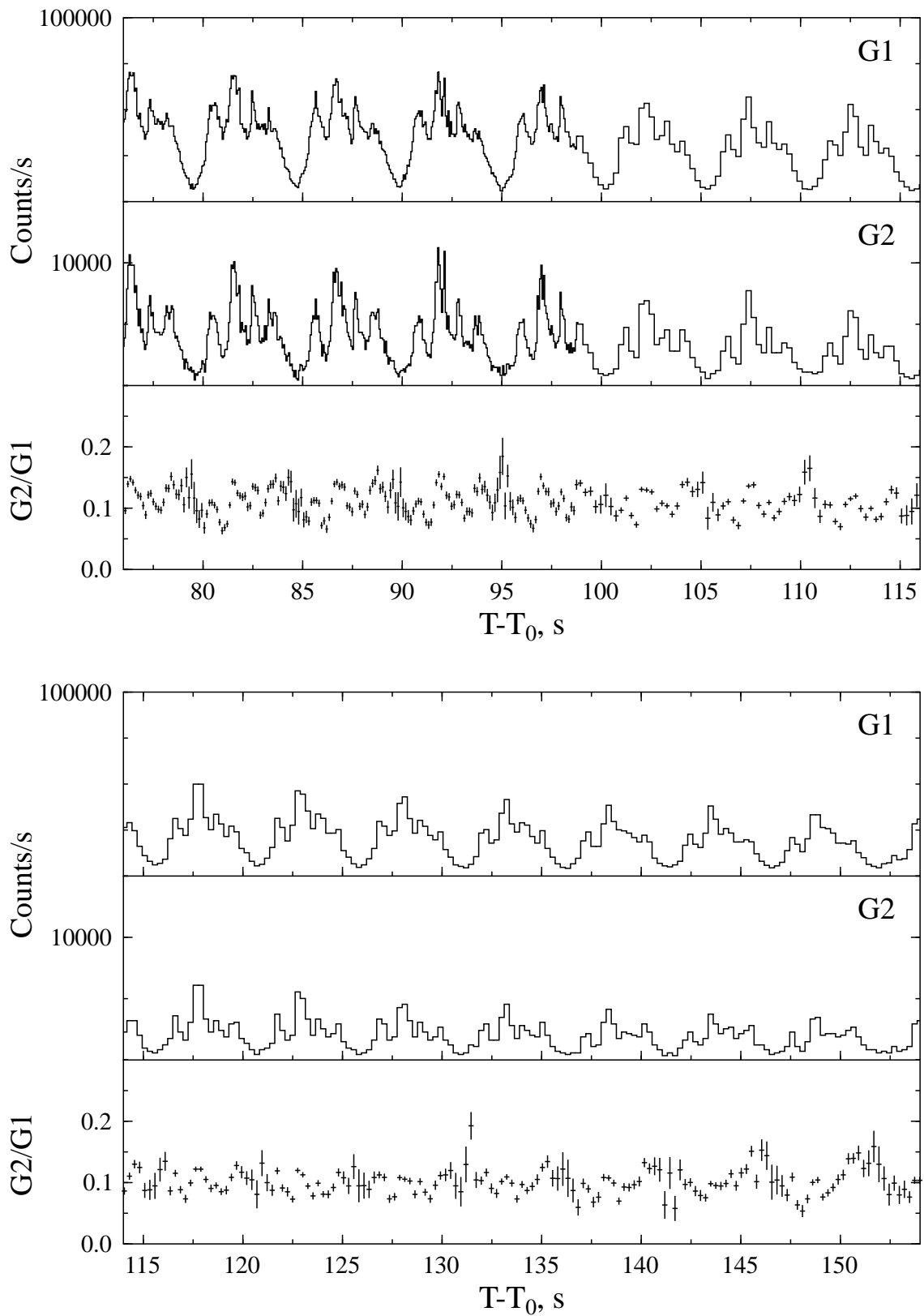
Fig. 3.30.— Pulsating tail of the 980827 outburst (continued).
