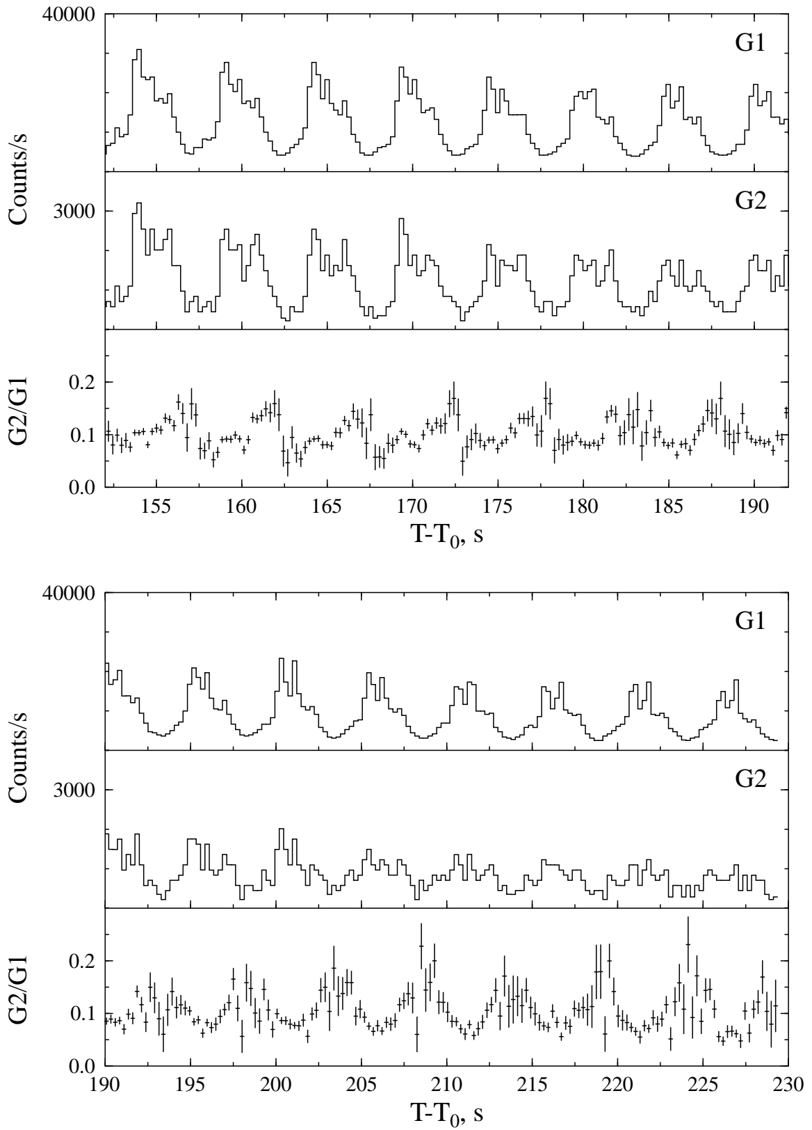
Fig. 3.31.— Pulsating tail of the 980827 outburst (continued).
