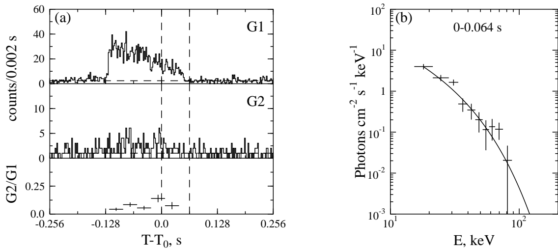
Fig. 3.41.— Event 980901c comprised a series of bursts. First burst caused a trigger.
