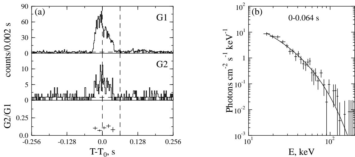
Fig. 3.55.— Event 981024 comprised a series of bursts. First burst caused a trigger.
