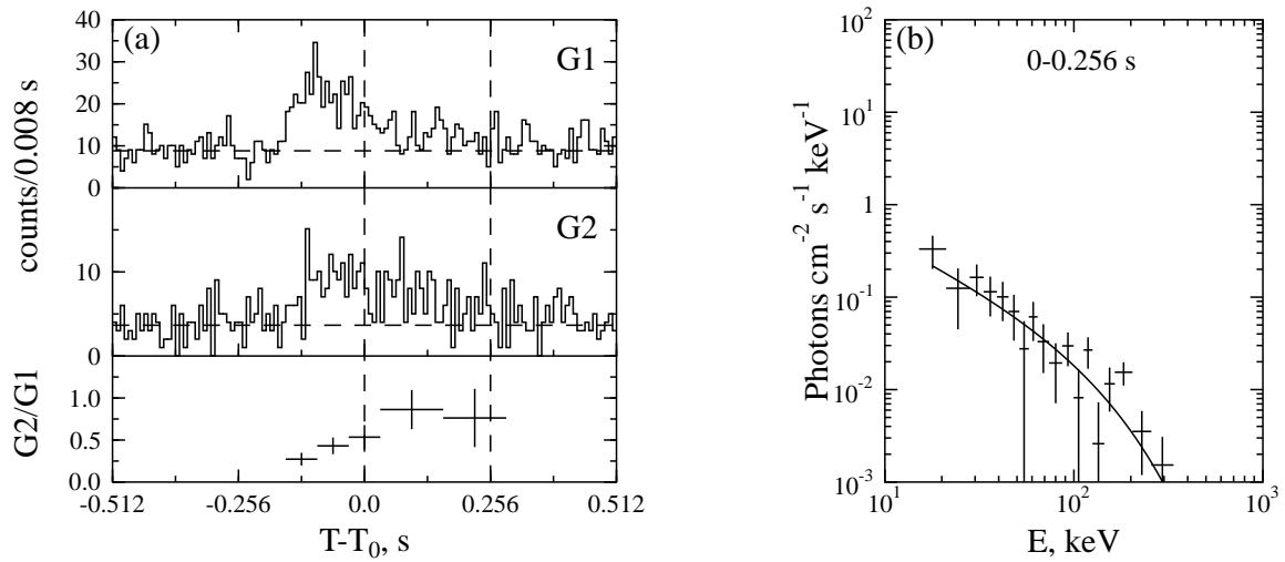
Fig. 3.54.— Burst 981022 exhibits an unusually hard energy spectrum ( kT \sim 100 keV) and a hardness-intensity anticorrelation (see Woods et al. 1999b). Another example of such a hard event is burst 990110. A similar hardness-intensity behaviour is also seen in the more common type of soft burst such as 980607a, 980821, 980530d.
