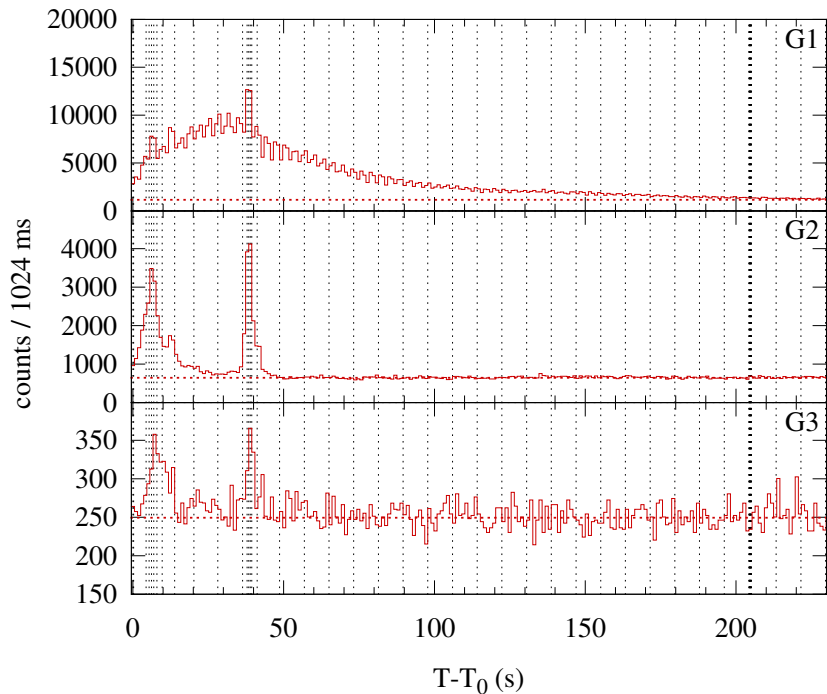
Konus-WIND S1 SOL1996-04-22T04:45 (M3.6) T 0 = 17109.241 s UT (04:45:09.241)
