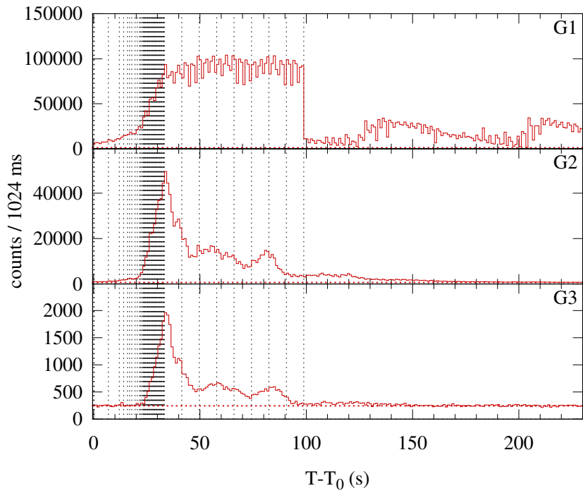
Konus-WIND S1 SOL1996-07-09T09:09 (X2.6) T_0 = 32941.340 s UT (09:09:01.340)
