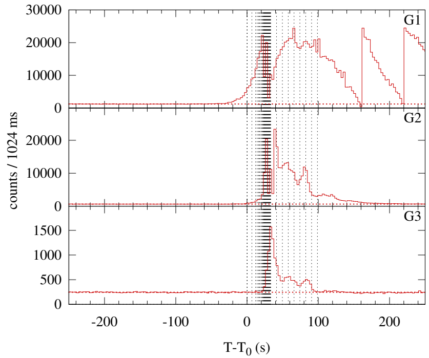
Konus-WIND S1 SOL1996-07-09T09:09 (X2.6) T_0 = 32941.340 s UT (09:09:01.340)
