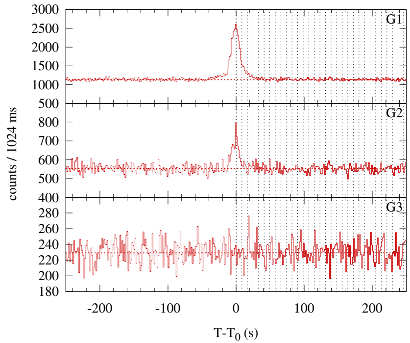
Konus-WIND S1 SOL1997-09-14T02:53 (C2.8) T_0 = 10409.698 s UT (02:53:29.698)
