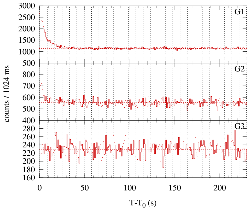
Konus-WIND S1 SOL1997-09-14T02:53 (C2.8) T_0 = 10409.698 s UT (02:53:29.698)
