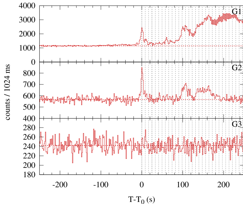
Konus-WIND S1 SOL1997-09-24T11:01 (M3.0) T_0 = 39677.294 s UT (11:01:17.294)
