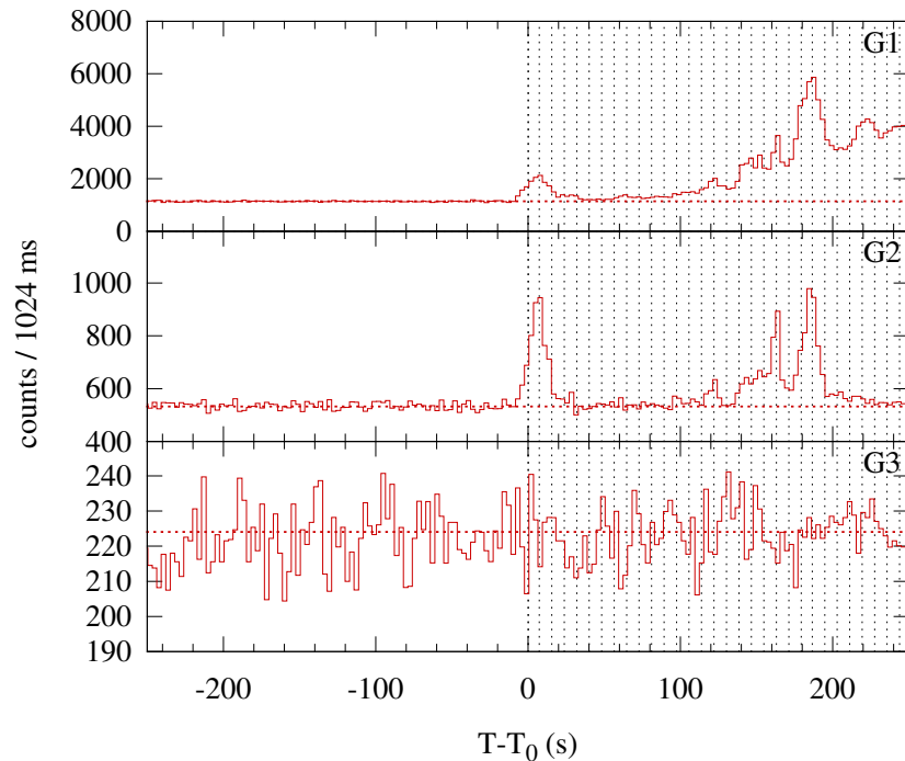
Konus-WIND S1 SOL1997-11-26T18:32 (M2.0) T_0 = 66725.621 s UT (18:32:05.621)
