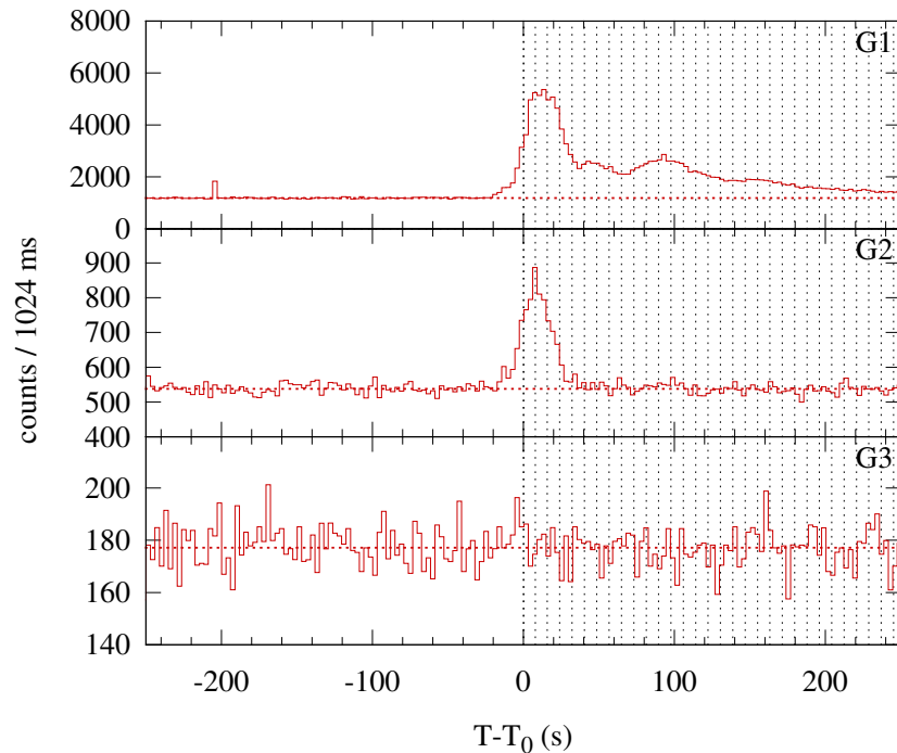
Konus-WIND S2 SOL1997-12-01T02:35 (M1.2) T 0 = 9305.728 s UT (02:35:05.728)
