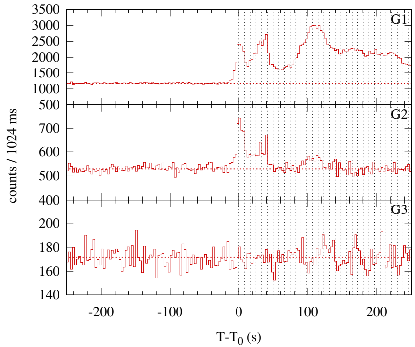
Konus-WIND S2 SOL1998-03-15T21:42 (M2.7) T 0 = 78139.785 s UT (21:42:19.785)
