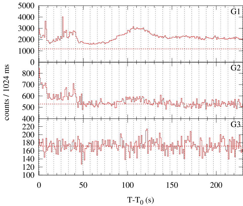
Konus-WIND S2 SOL1998-03-15T21:42 (M2.7) T 0 = 78139.785 s UT (21:42:19.785)
