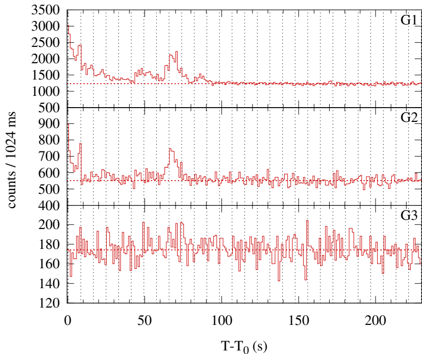
Konus-WIND S2 SOL1998-04-09T18:13 (C2.9) T 0 = 65609.207 s UT (18:13:29.207)
