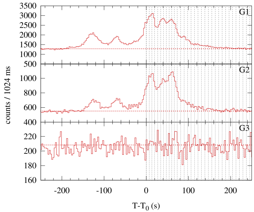
Konus-WIND S2 SOL1998-05-02T04:56 (C5.4) T 0 = 17777.419 s UT (04:56:17.419)
