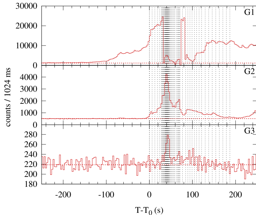
Konus-WIND S1 SOL1998-05-06T08:02 (X2.7) T 0 = 28973.411 s UT (08:02:53.411)
