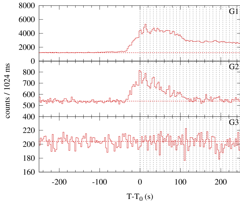
Konus-WIND S2 SOL1998-05-08T01:57 (M3.1) T_0 = 7038.426 s UT (01:57:18.426)
