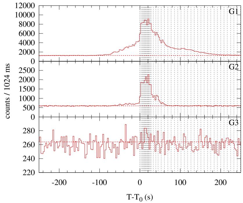
Konus-WIND S2 SOL1998-05-10T13:18 (M3.9) T_0 = 47906.603 s UT (13:18:26.603)
