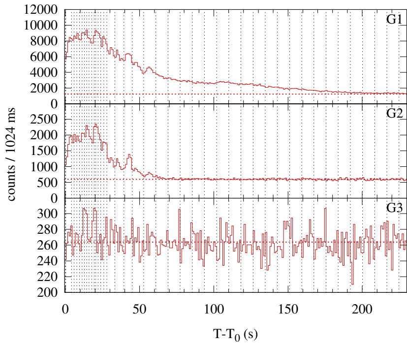
Konus-WIND S2 SOL1998-05-10T13:18 (M3.9) T_0 = 47906.603 s UT (13:18:26.603)
