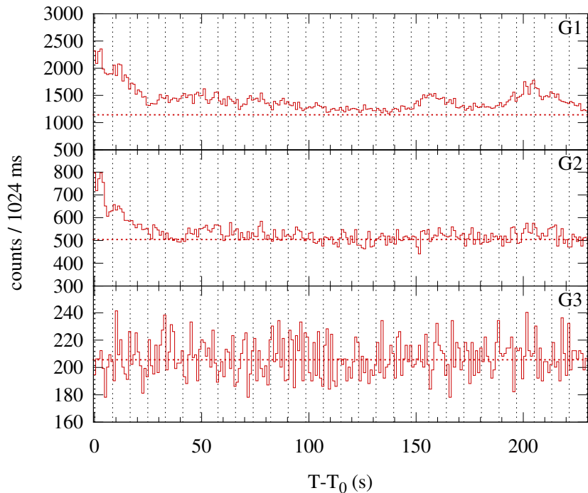
Konus-WIND S1 SOL1998-05-28T19:02 (C8.7) T 0 = 68574.765 s UT (19:02:54.765)
