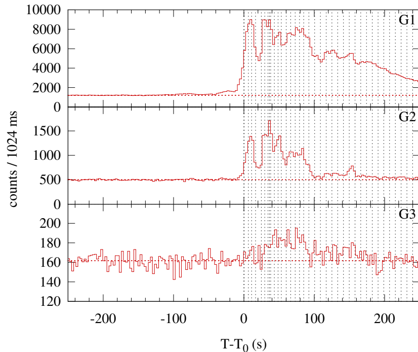
Konus-WIND S2 SOL1998-05-29T00:55 (M6.7) T 0 = 3334.440 s UT (00:55:34.440)
