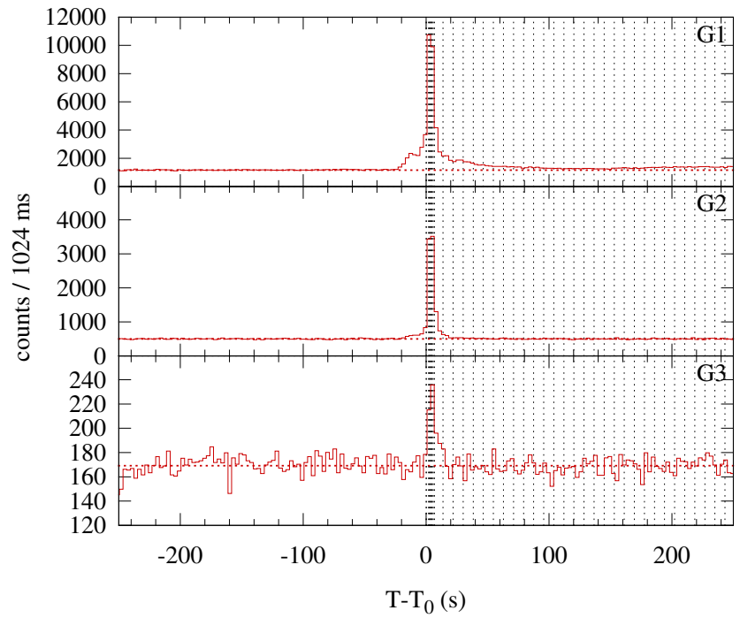
Konus-WIND S2 SOL1998-06-13T04:18 (M1.9) T 0 = 15510.172 s UT (04:18:30.172)
