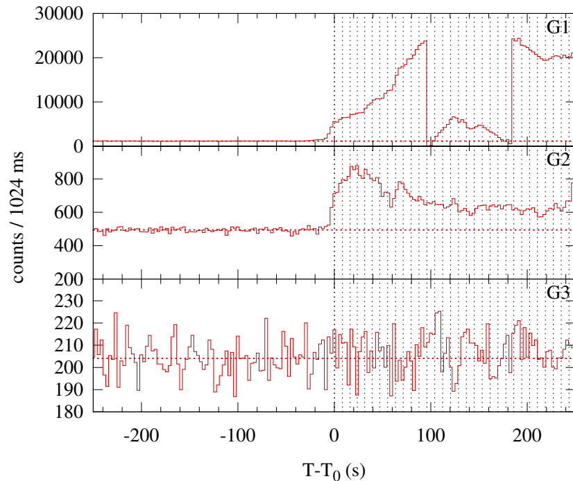
Konus-WIND S1 SOL1998-08-17T21:13 (X1.2) T 0 = 76411.445 s UT (21:13:31.445)
