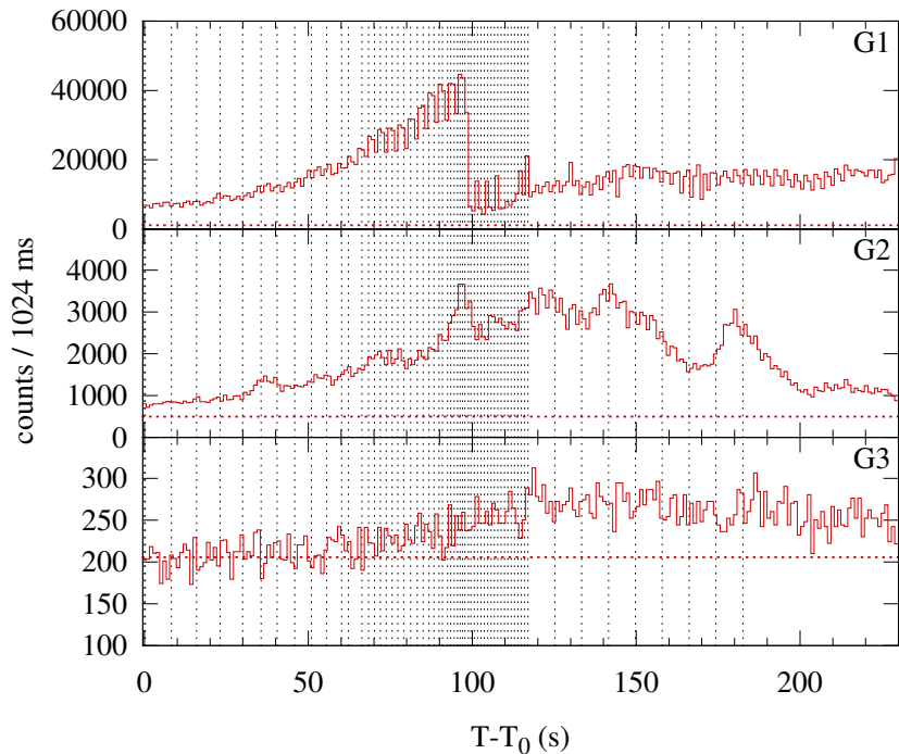
Konus-WIND S1 SOL1998-08-18T08:18 (X2.8) T 0 = 29881.433 s UT (08:18:01.433)
