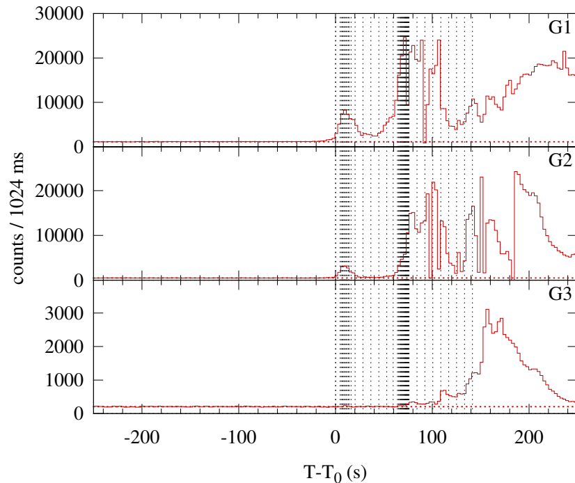
Konus-WIND S1 SOL1998-08-18T22:13 (X4.9) T_0 = 79990.994 s UT (22:13:10.994)
