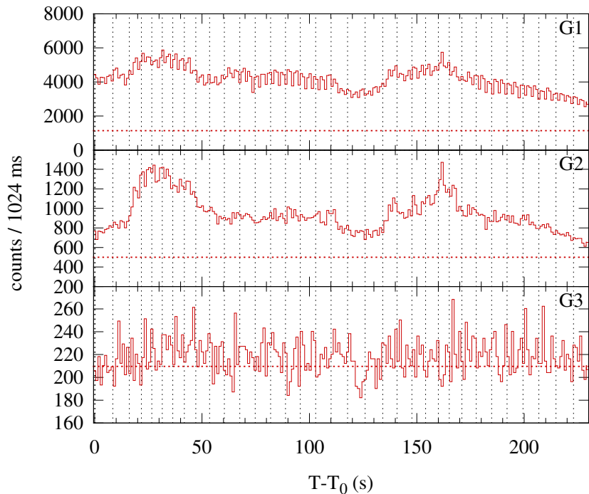
Konus-WIND S1 SOL1998-08-19T14:09 (M3.0) T_0 = 50996.102 s UT (14:09:56.102)
