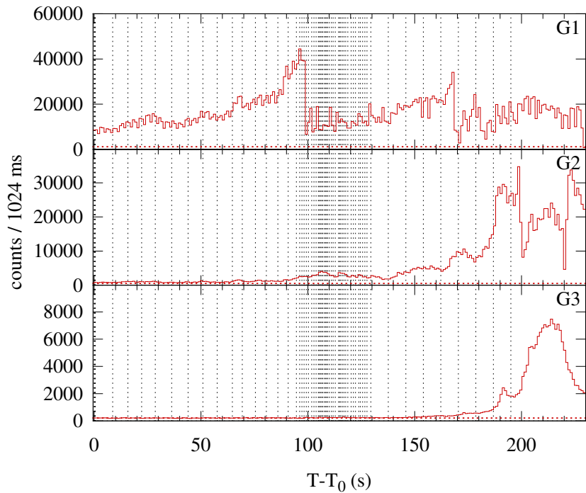
Konus-WIND S1 SOL1998-08-19T21:40 (X3.9) T_0 = 78002.352 s UT (21:40:02.352)
