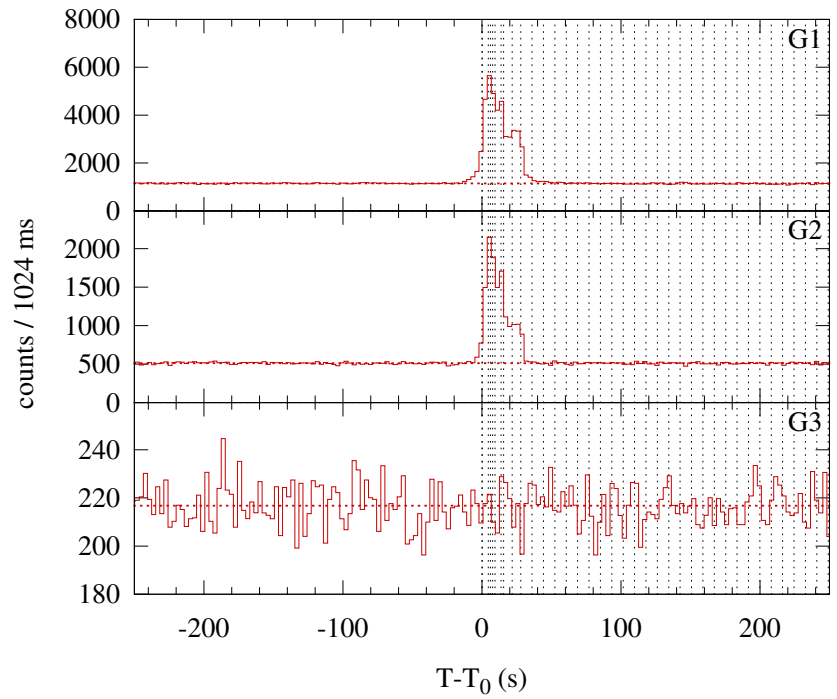
Konus-WIND S1 SOL1998-08-22T15:05 (C1.9) T_0 = 54328.734 s UT (15:05:28.734)
