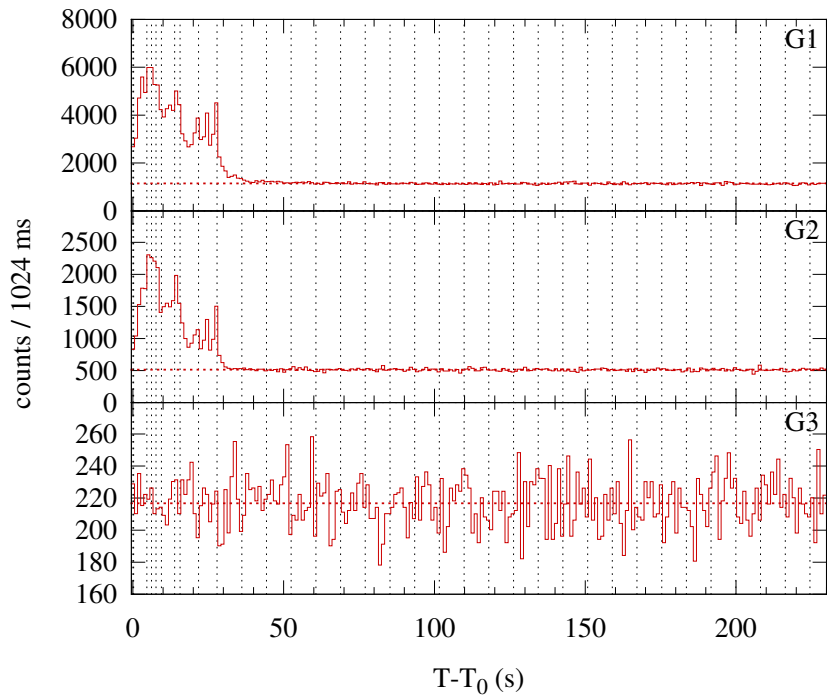
Konus-WIND S1 SOL1998-08-22T15:05 (C1.9) T_0 = 54328.734 s UT (15:05:28.734)
