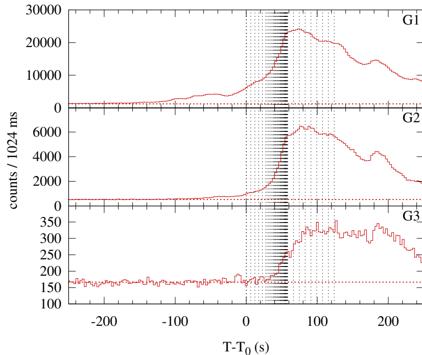
Konus-WIND S2 SOL1998-08-24T22:01 (X1.0) T_0 = 79311.773 s UT (22:01:51.773)
