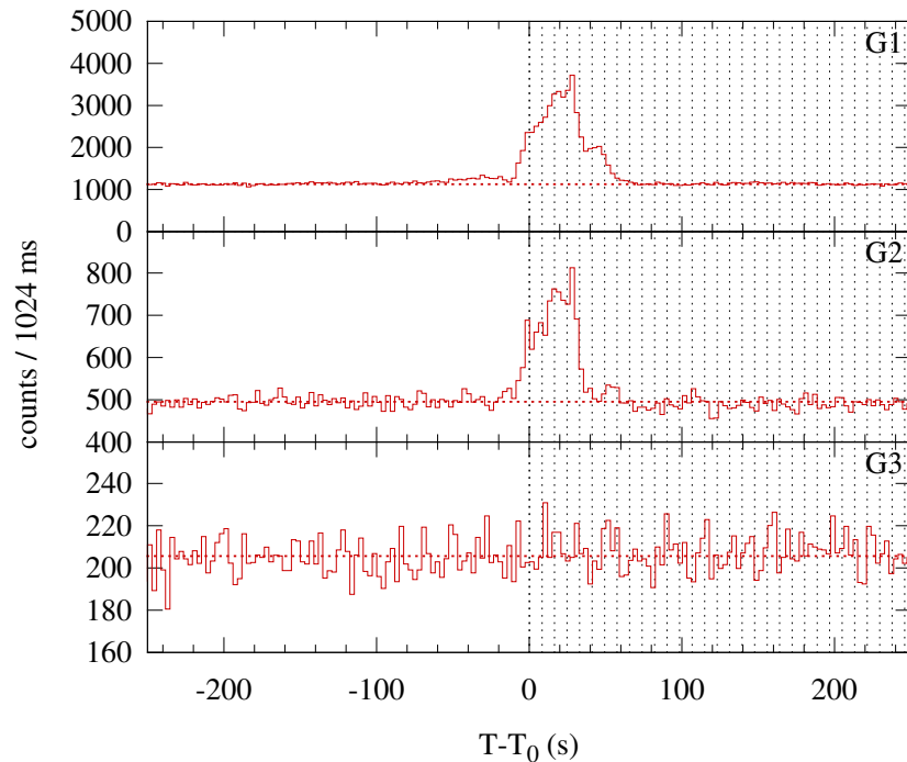
Konus-WIND S1 SOL1998-09-06T02:12 (C2.3) T 0 = 7930.664 s UT (02:12:10.664)
