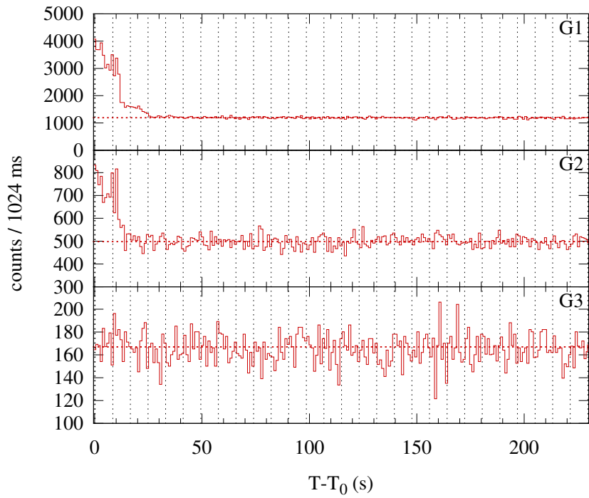
Konus-WIND S2 SOL1998-09-06T11:06 (C1.3) T 0 = 39970.623 s UT (11:06:10.623)
