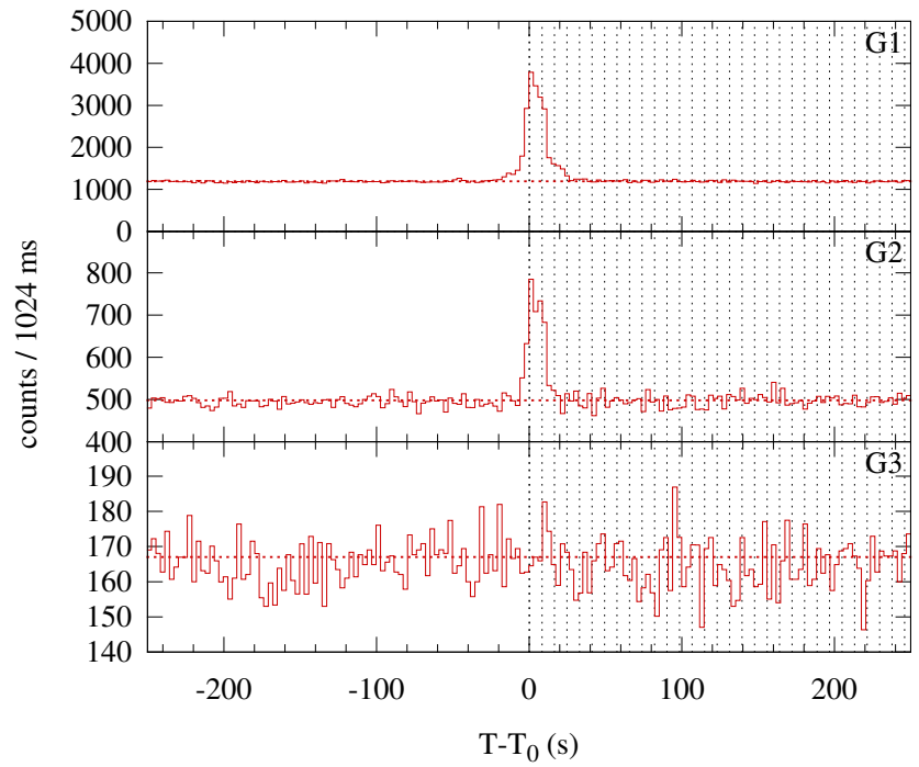
Konus-WIND S2 SOL1998-09-06T11:06 (C1.3) T 0 = 39970.623 s UT (11:06:10.623)
