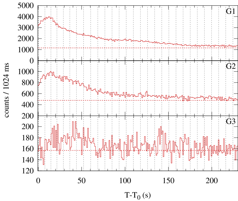
Konus-WIND S2 SOL1998-09-20T02:40 (M1.8) T_0 = 9602.829 s UT (02:40:02.829)
