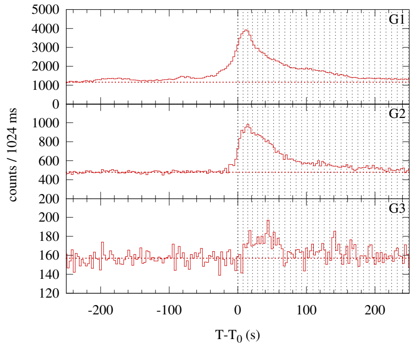
Konus-WIND S2 SOL1998-09-20T02:40 (M1.8) T_0 = 9602.829 s UT (02:40:02.829)
