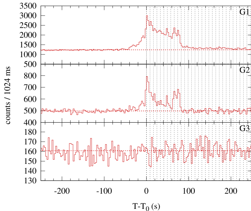
Konus-WIND S2 SOL1998-09-27T23:38 (C6.0) T_0 = 85129.320 s UT (23:38:49.320)
