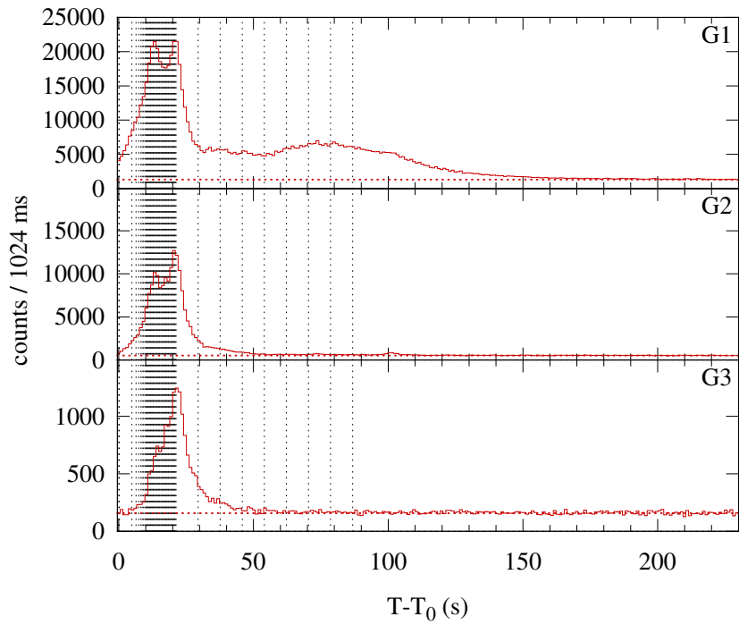
Konus-WIND S2 SOL1998-09-28T06:52 (M3.5) T 0 = 24765.356 s UT (06:52:45.356)
