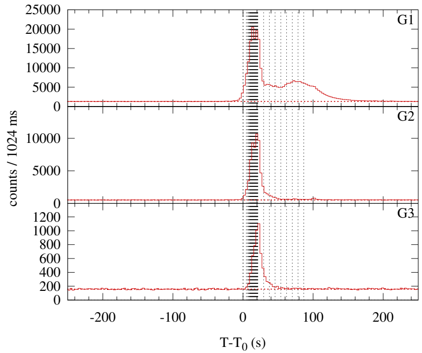
Konus-WIND S2 SOL1998-09-28T06:52 (M3.5) T 0 = 24765.356 s UT (06:52:45.356)
