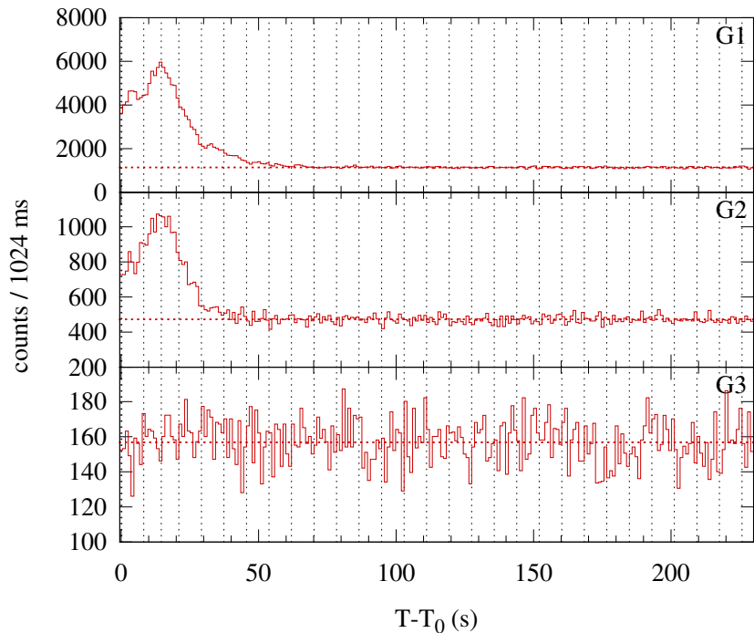
Konus-WIND S2 SOL1998-10-28T13:15 (C2.3) T 0 = 47730.275 s UT (13:15:30.275)
