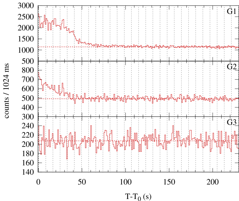
Konus-WIND S1 SOL1998-11-06T08:30 (C3.5) T 0 = 30648.323 s UT (08:30:48.323)
