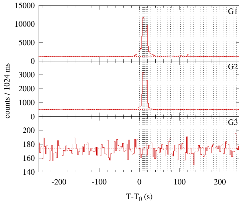
Konus-WIND S2 SOL1998-11-06T12:04 (C6.4) T 0 = 43445.554 s UT (12:04:05.554)
