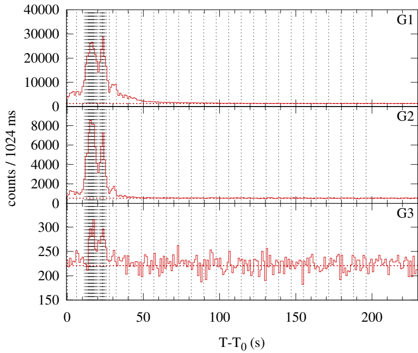
Konus-WIND S1 SOL1998-11-06T15:10 (M1.7) T 0 = 54621.278 s UT (15:10:21.278)
