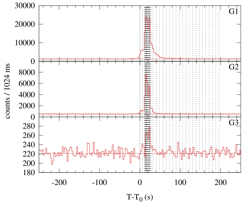
Konus-WIND S1 SOL1998-11-06T15:10 (M1.7) T 0 = 54621.278 s UT (15:10:21.278)
