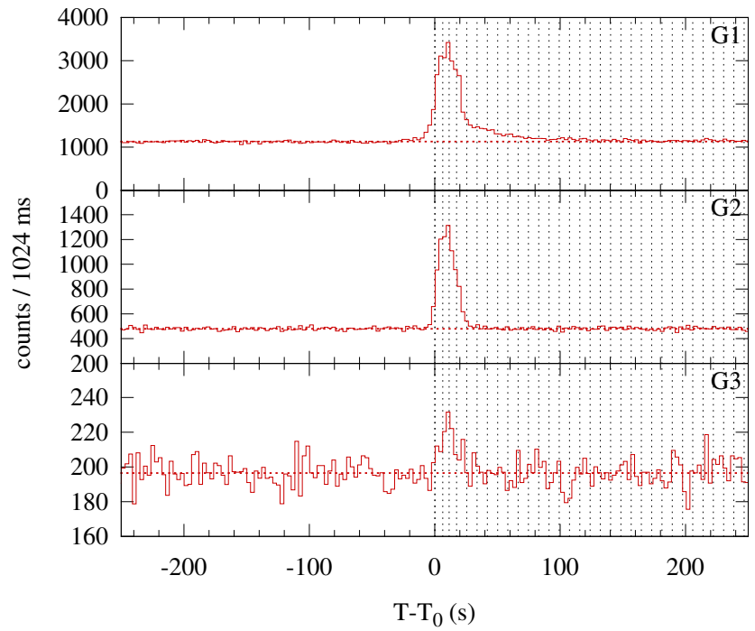
Konus-WIND S1 SOL1998-11-12T05:26 (M1.0) T 0 = 19613.864 s UT (05:26:53.864)
