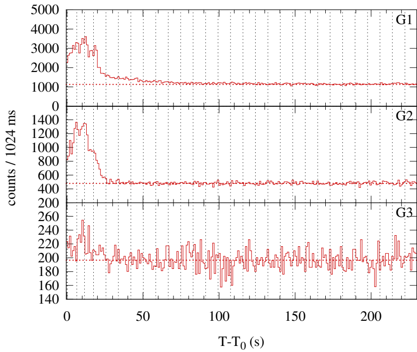
Konus-WIND S1 SOL1998-11-12T05:26 (M1.0) T 0 = 19613.864 s UT (05:26:53.864)
