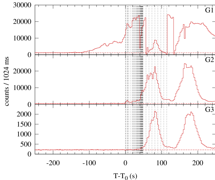
Konus-WIND S1 SOL1998-11-22T06:36 (X3.7) T 0 = 23793.669 s UT (06:36:33.669)
