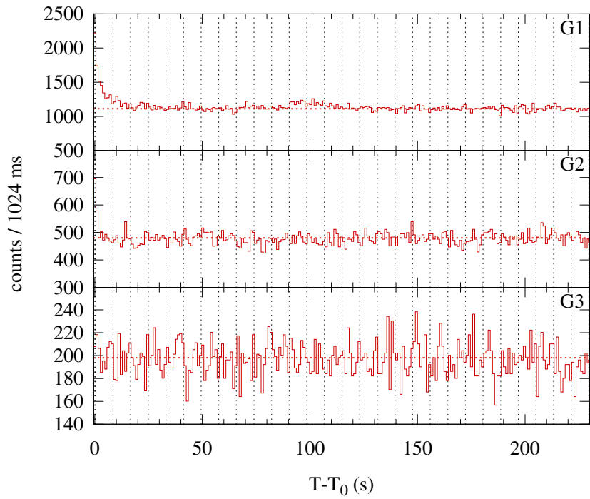
Konus-WIND S1 SOL1998-11-30T10:15 (C3.7) T_0 = 36949.357 s UT (10:15:49.357)
