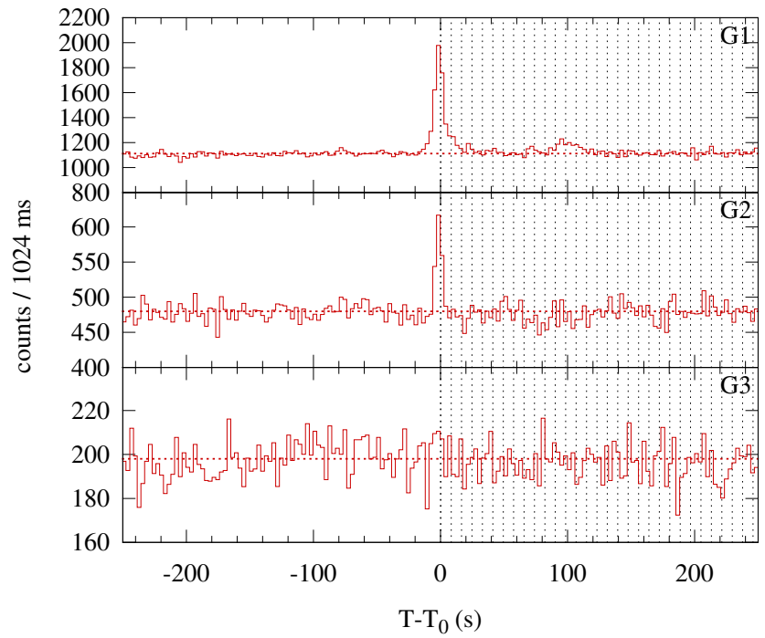
Konus-WIND S1 SOL1998-11-30T10:15 (C3.7) T_0 = 36949.357 s UT (10:15:49.357)
