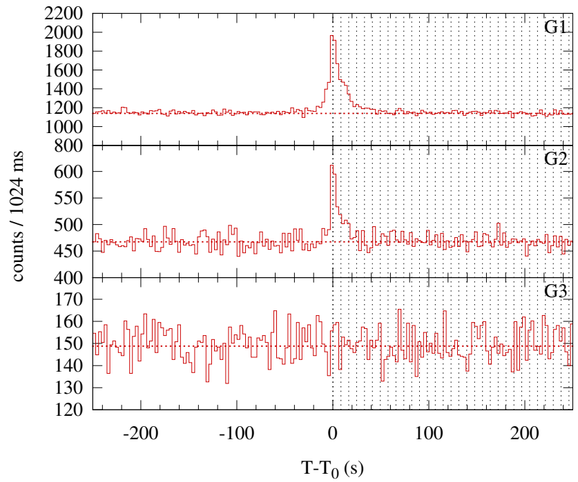
Konus-WIND S2 SOL1998-12-13T05:15 (C3.0) T_0 = 18914.551 s UT (05:15:14.551)
