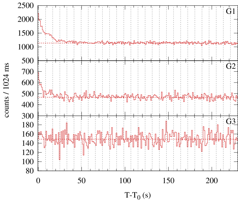
Konus-WIND S2 SOL1998-12-13T05:15 (C3.0) T_0 = 18914.551 s UT (05:15:14.551)
