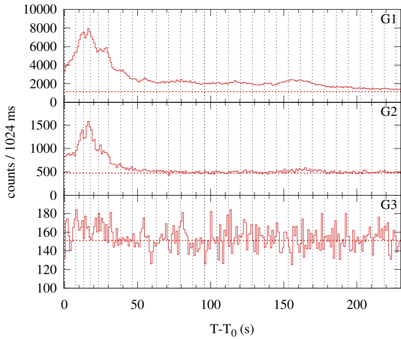
Konus-WIND S2 SOL1998-12-17T07:42 (M3.2) T_0 = 27779.899 s UT (07:42:59.899)
