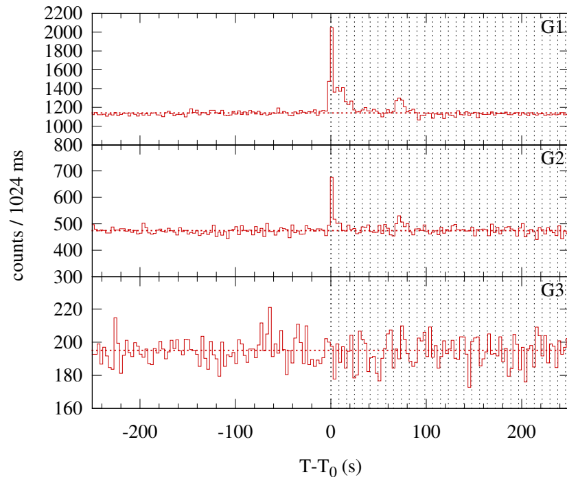
Konus-WIND S1 SOL1998-12-18T12:51 (C2.9) T 0 = 46273.605 s UT (12:51:13.605)
