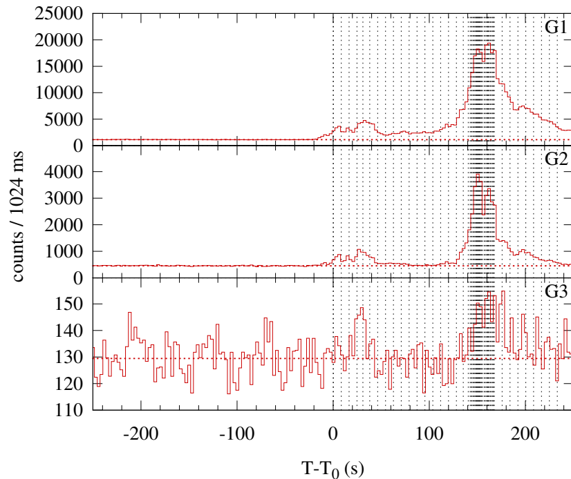
Konus-WIND S2 SOL2000-01-12T01:33 (M2.8) T_0 = 5607.890 s UT (01:33:27.890)
