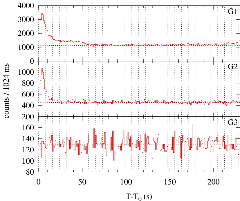
Konus-WIND S2 SOL2000-01-12T20:41 (M1.1) T 0 = 74477.37 s UT (20:41:17.37)
