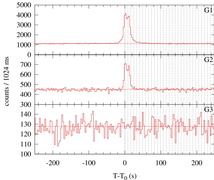
Konus-WIND S2 SOL2000-01-15T01:58 (C4.0) T_0 = 7117.394 s UT (01:58:37.394)
