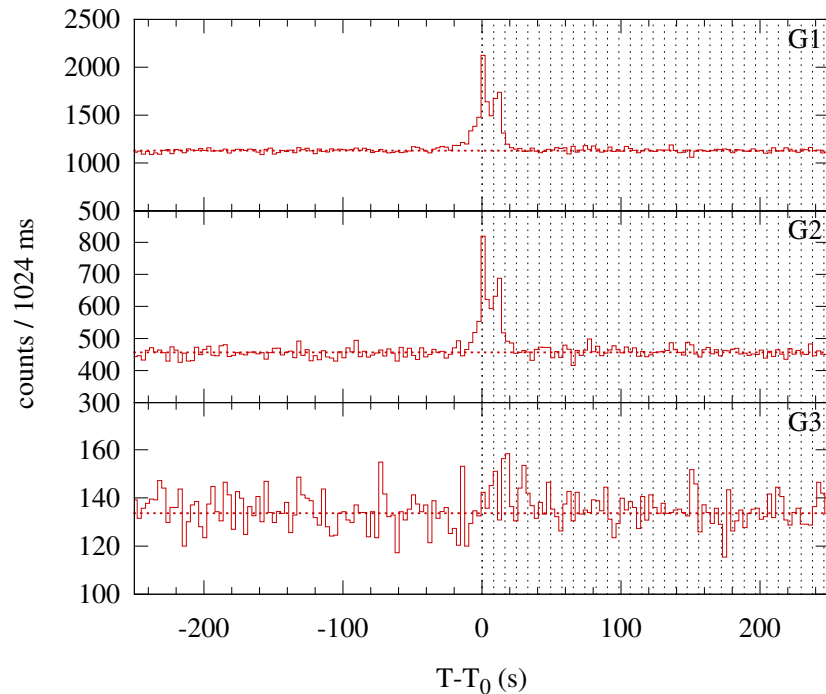
Konus-WIND S2 SOL2000-01-19T11:19 (C1.3) T_0 = 40783.666 s UT (11:19:43.666)
