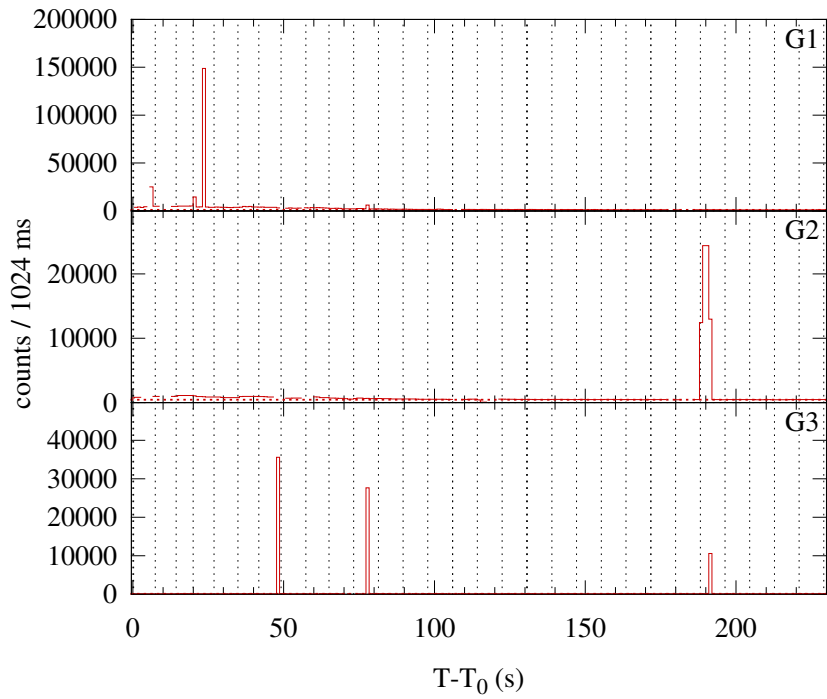
Konus-WIND S2 SOL2000-02-03T19:58 (C8.4) T_0 = 71904.972 s UT (19:58:24.972)
