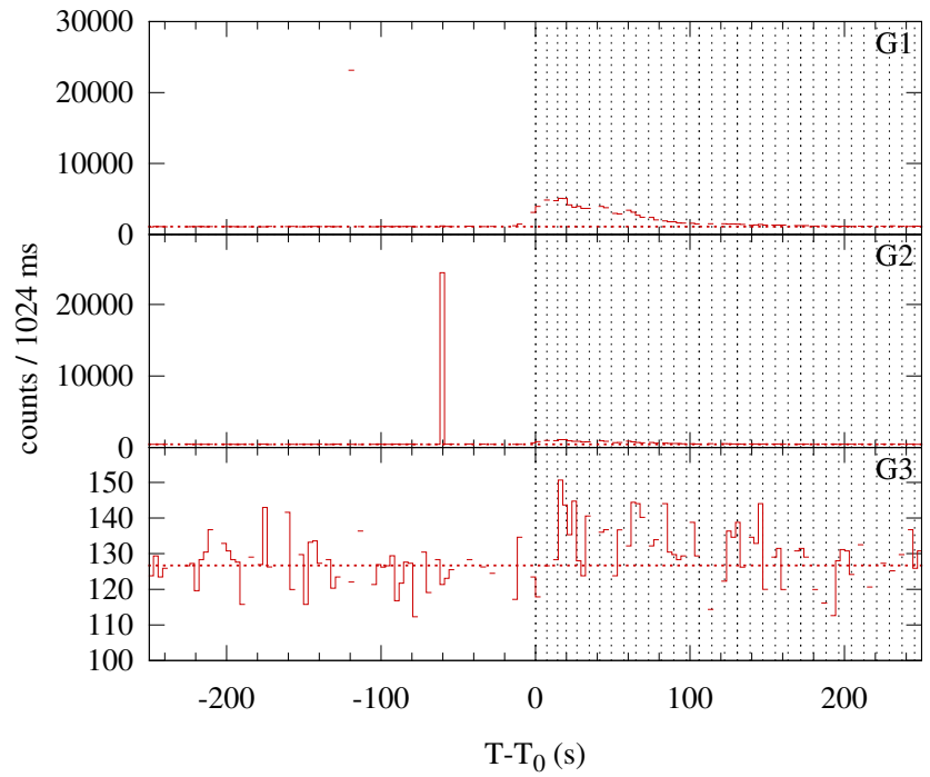
Konus-WIND S2 SOL2000-02-03T19:58 (C8.4) T_0 = 71904.972 s UT (19:58:24.972)
