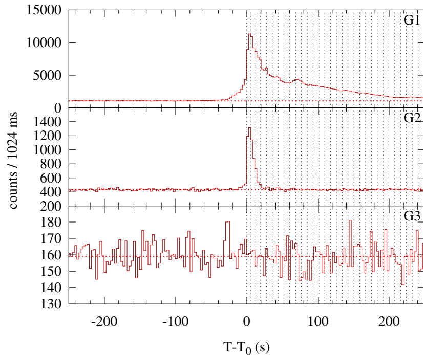
Konus-WIND S1 SOL2000-02-04T09:15 (M3.0) T 0 = 33304.154 s UT (09:15:04.154)
