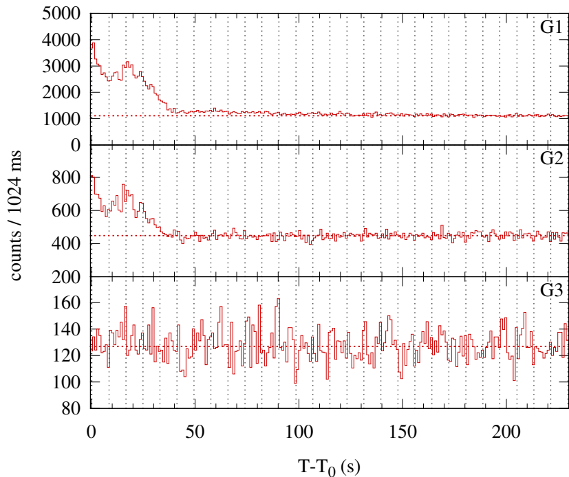
Konus-WIND S2 SOL2000-02-04T17:59 (C4.9) T 0 = 64760.475 s UT (17:59:20.475)
