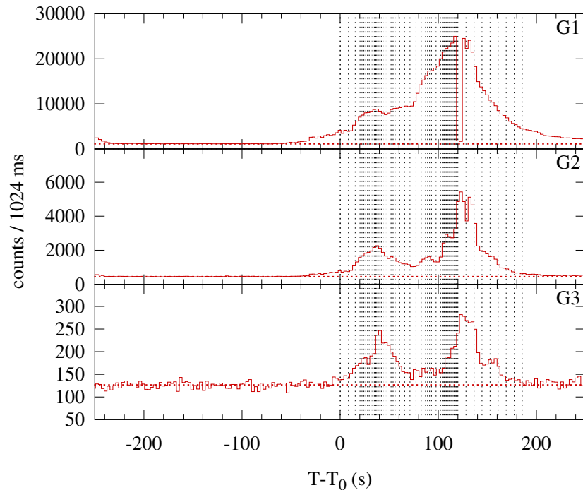
Konus-WIND S2 SOL2000-02-05T19:25 (X1.2) T 0 = 69938.494 s UT (19:25:38.494)
