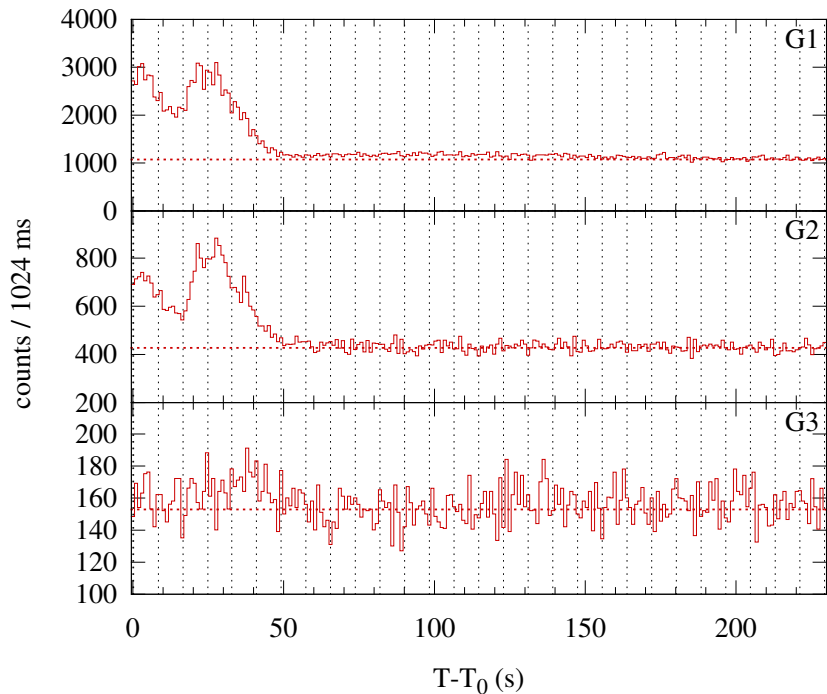
Konus-WIND S1 SOL2000-02-24T01:06 (M1.1) T 0 = 4006.513 s UT (01:06:46.513)
